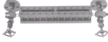
Reflex type gauge glass
